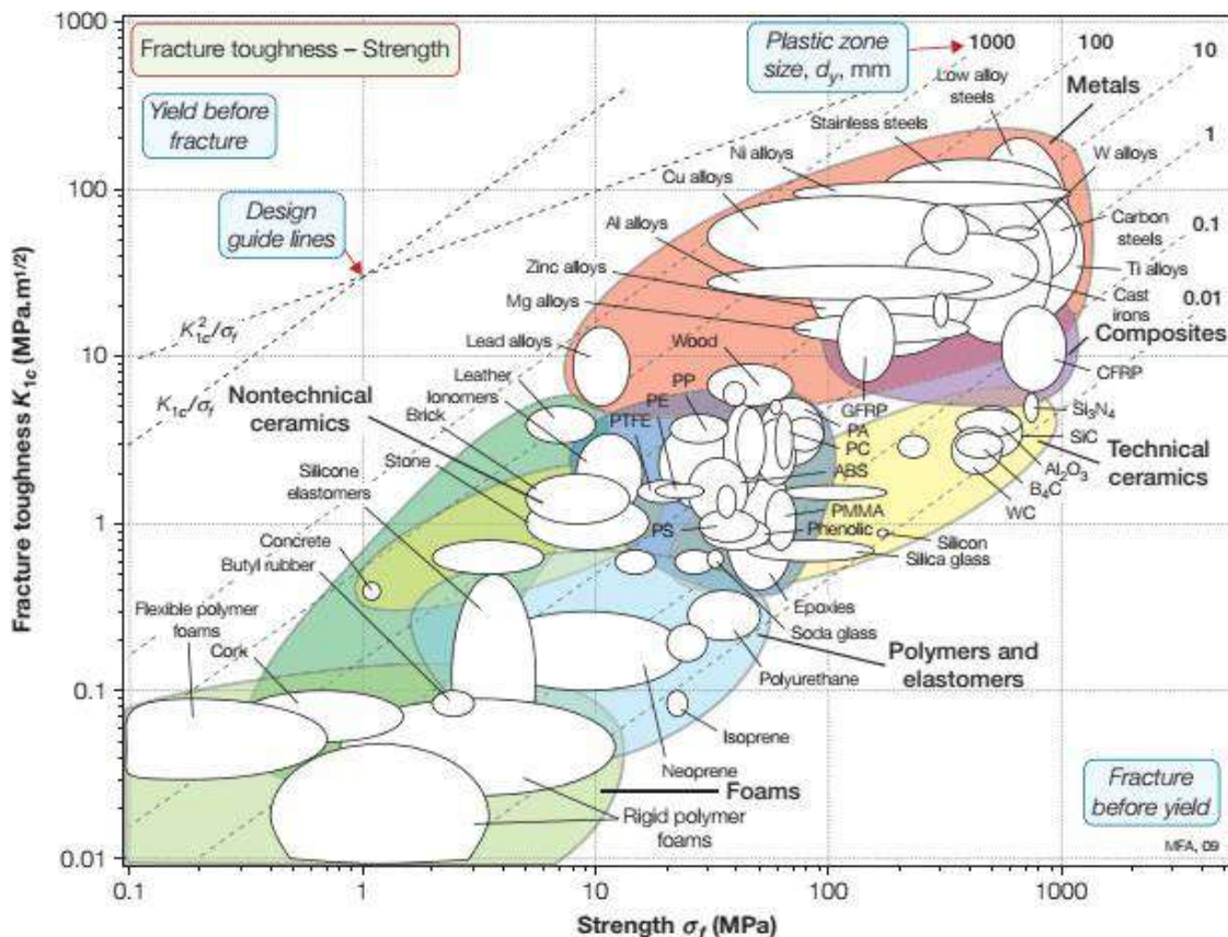
Figure 18: Fracture toughness K_{Ic} plotted against strength \sigma_f . The contours show the value of K_{Ic}^2/\pi\sigma_f^2 —roughly the diameter d_y of the process zone at a crack tip. The design guide lines are used in selecting materials for damage-tolerant design.
