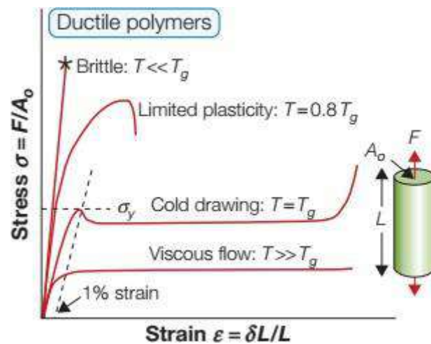
Figure 7: Stress-strain curves for a polymer below, at, and above its glass transition temperature, T_g .
