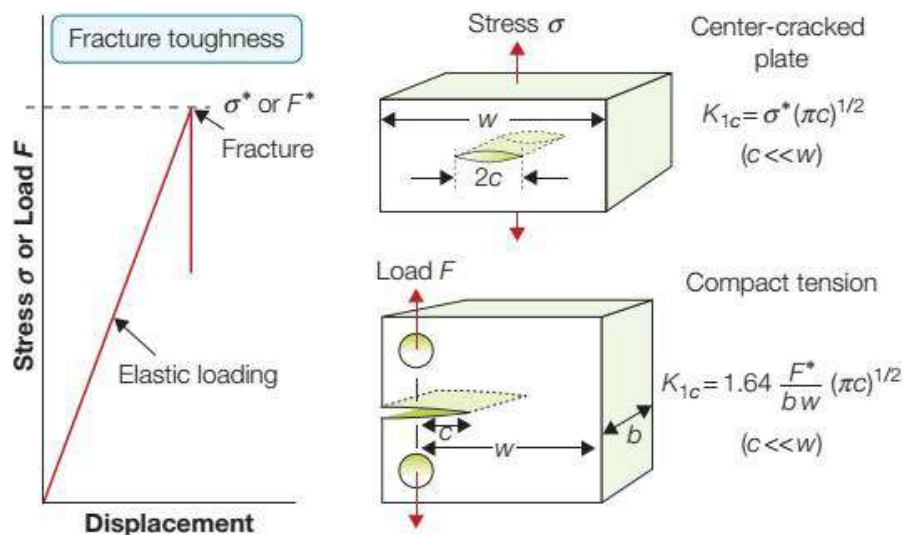
Figure 11: The fracture toughness, K_{1c} , measures the resistance to the propagation of a crack. The test specimen containing a crack of length 2c fails at stress \sigma^* . The fracture
