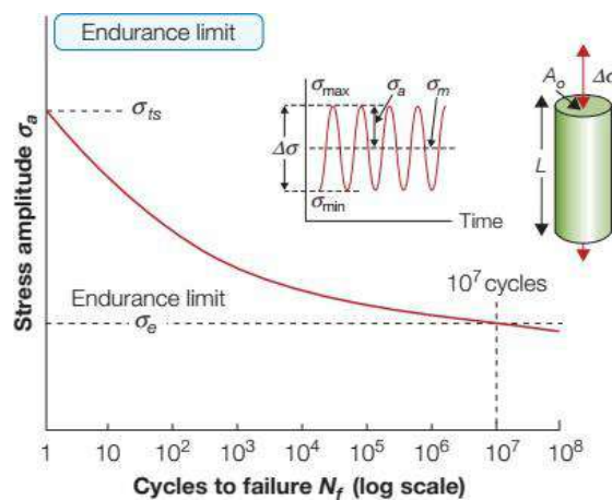
Figure 10: Fatigue curve
