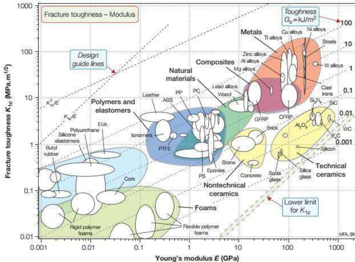
Figure 17: Fracture toughness K_{Ic} plotted against Young's modulus E . The family of lines is of constant K_{Ic}^2/E (approximately G_{Ic} , the fracture energy or toughness). These, and the guide line of constant K_{Ic}/E , help in design against fracture. The shaded band shows the lower limit for K_{Ic} .
